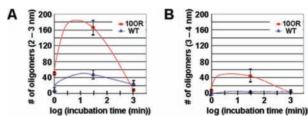
Figure 5. Kinetics of oligomerization. (A,B) Number of oligomers with heights between (A) 2–3 nm and (B) 3–4 nm versus incubation time. Red, 10OR; blue, WT.
