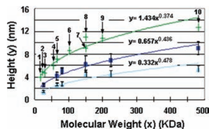
Figure 2. Heights of marker proteins and newly formed 10OR oligomers (at t = 0^+ min) deposited on mica versus molecular weights. Heights were measured from the surface of mica to the top of protein particles. Light blue \blacktriangle : ex situ curve where, from left to right, points are for 10OR monomers (26.8 KDa), BSA monomers ( \sim 66 KDa), majority of newly formed 10OR oligomers (seeds) such as those marked with yellow arrowheads in Figure 1, C and D assuming they are trimers (80.4 KDa), IgG monomers ( \sim 150 KDa), MAS monomers ( \sim 224 KDa), and Apoferritin monomers ( \sim 481.2 KDa). Dark blue \blacksquare : in situ curve where order left to right is the same as for ex situ curve. Green + : hydrodynamic diameters. Numbers indicate: 1, myoglobin monomer (16.9 KDa); 32 2, WT monomer (22.8 KDa); 33 3, carbonic anhydrase monomer (29 KDa); 32 4, yeast triosephosphate isomerase dimer ( \sim 56 KDa); 34 5, BSA monomer; 32 6, hexokinase monomer (102 KDa) (Malvern Instruments); 7, alcohol dehydrogenase dimer (150 KDa); 32 8, IgG monomer; 35 9, \beta -amylase monomer (200 KDa); 32 10, apoferritin monomer. 36 Error bars represent \pm one standard deviation.
